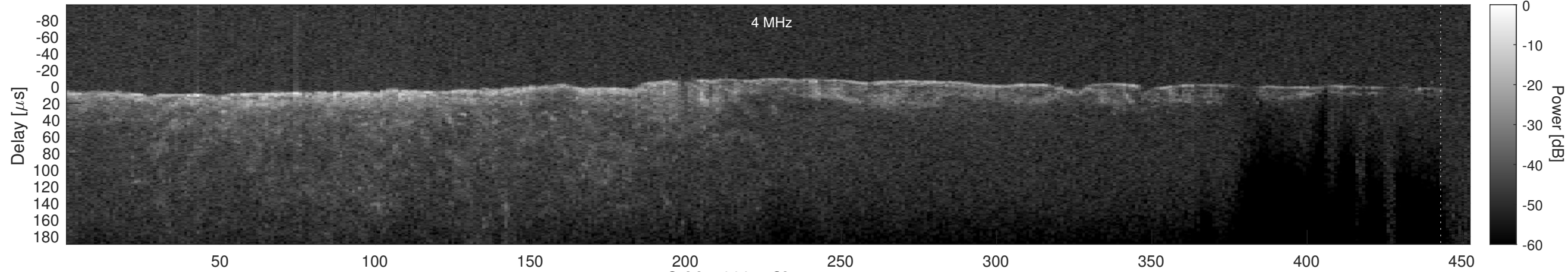
Orbit 19031, Cluttergram
