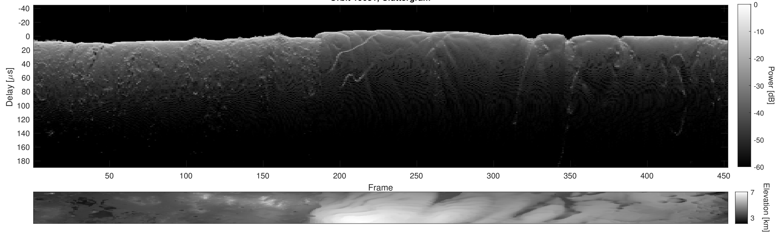
Orbit 19031, Cluttergram
