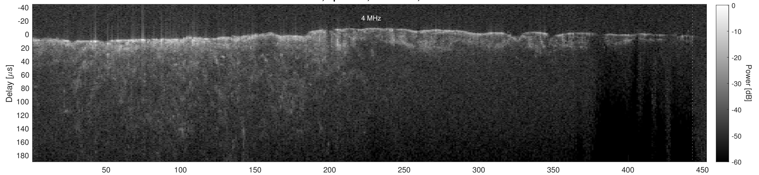
Orbit 19031, Cluttergram
