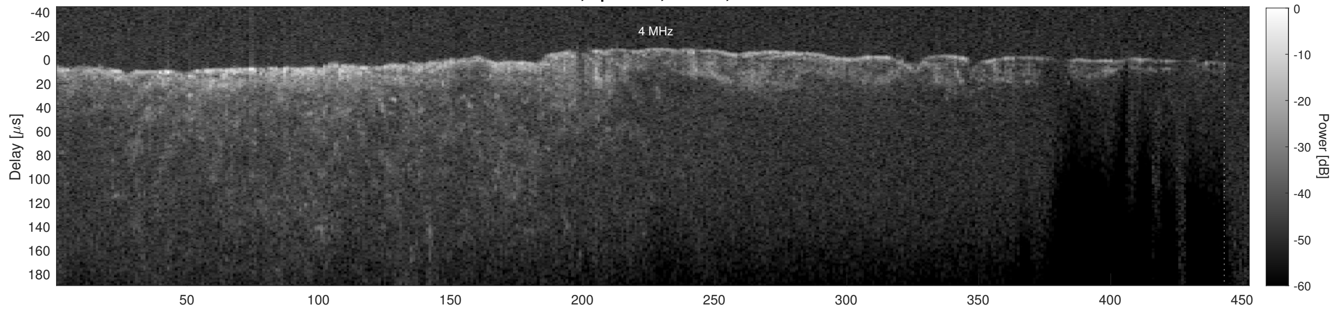
Orbit 19031, Cluttergram
