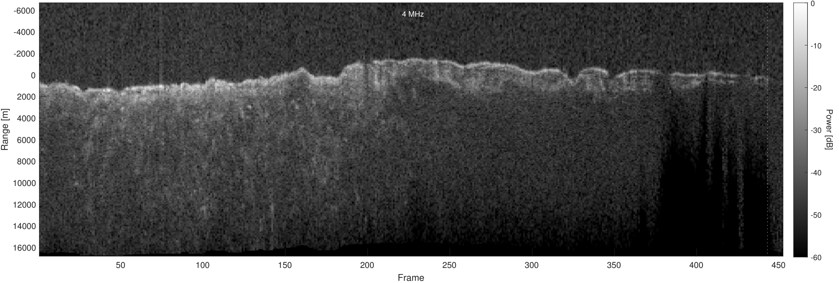
Orbit 19031, Optimized, Window, Depth-Corrected, Channel 2
