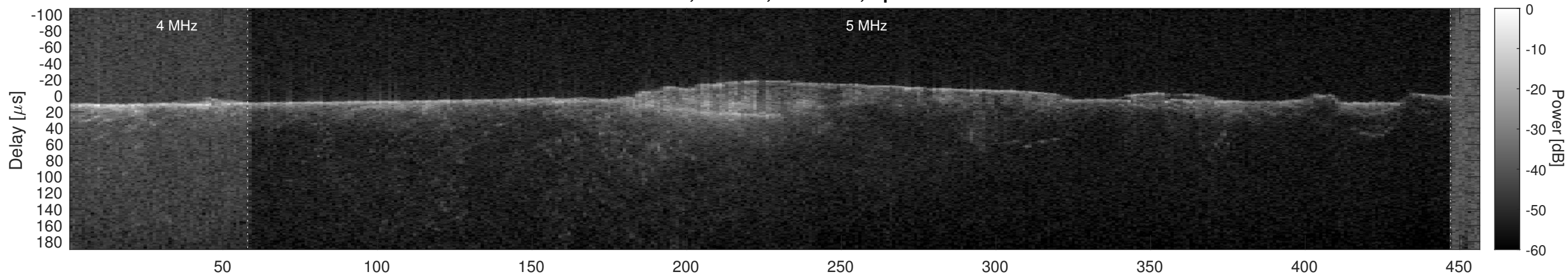
Orbit 19035, Cluttergram
