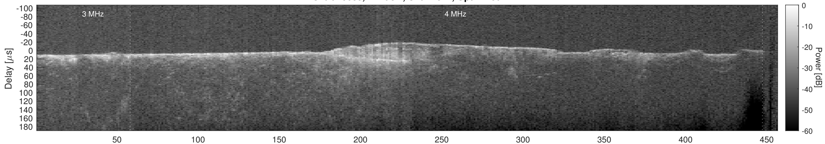
Orbit 19035, Cluttergram
