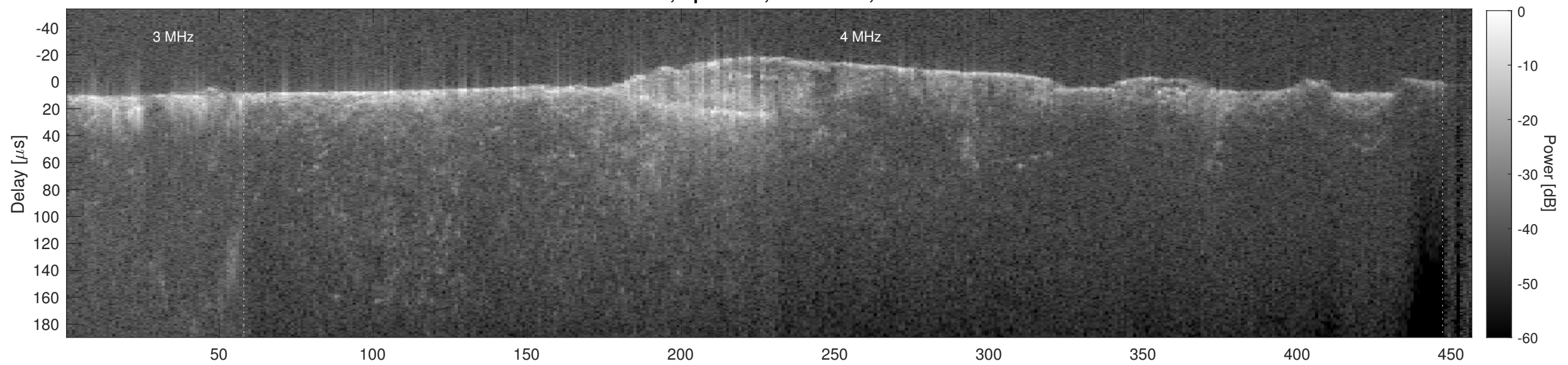
Orbit 19035, Cluttergram
