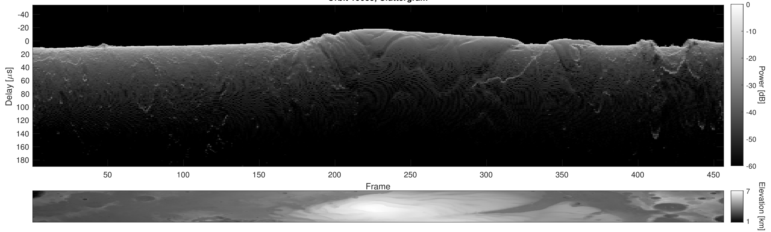
Orbit 19035, Cluttergram
