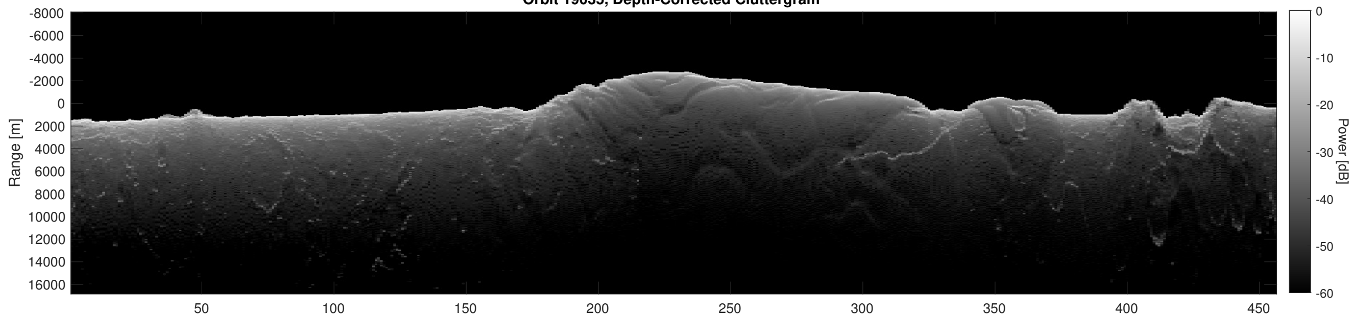
Orbit 19035, Depth-Corrected Cluttergram
