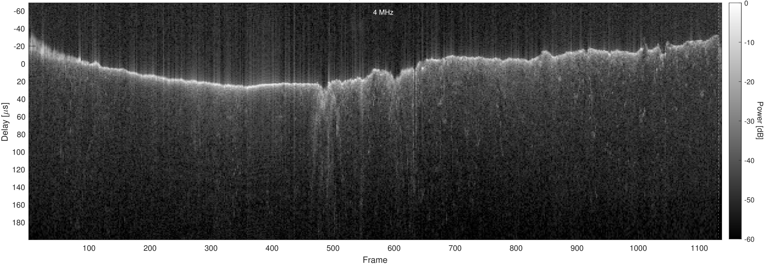
Orbit 19678, Chapman, No Window, Channel 2
