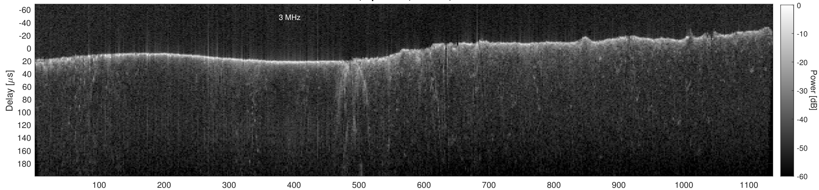
Orbit 19678, Cluttergram
