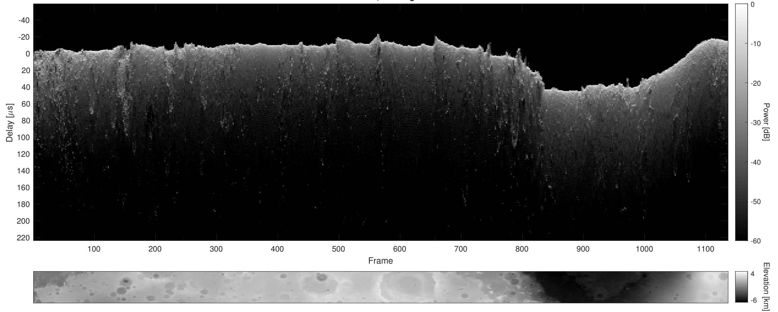
Orbit 19679, Cluttergram
