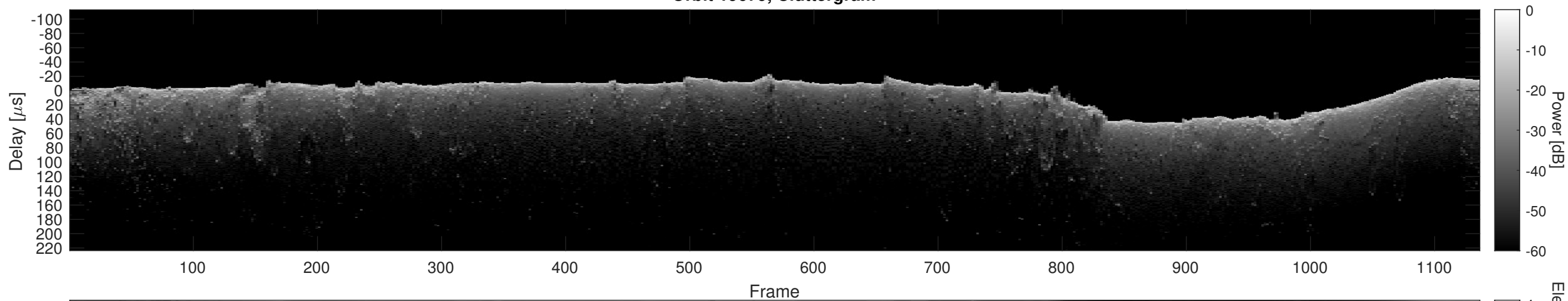
Orbit 19679, Cluttergram
