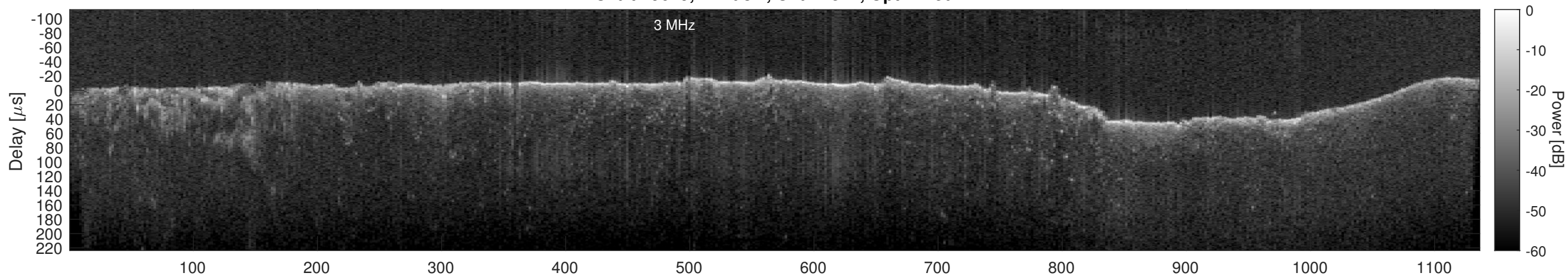
Orbit 19679, Cluttergram
