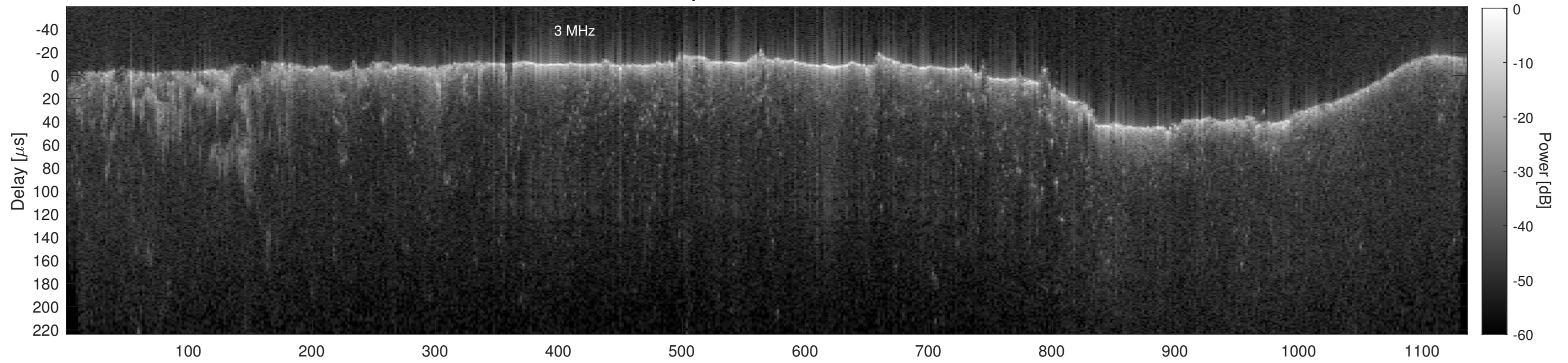
Orbit 19679, Cluttergram
