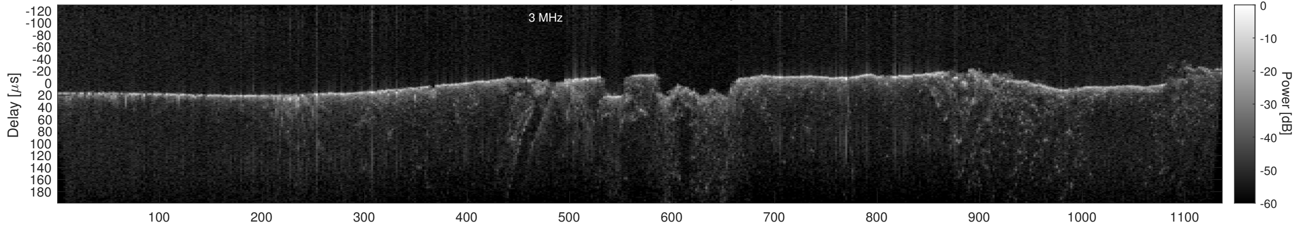
Orbit 19680, Cluttergram
