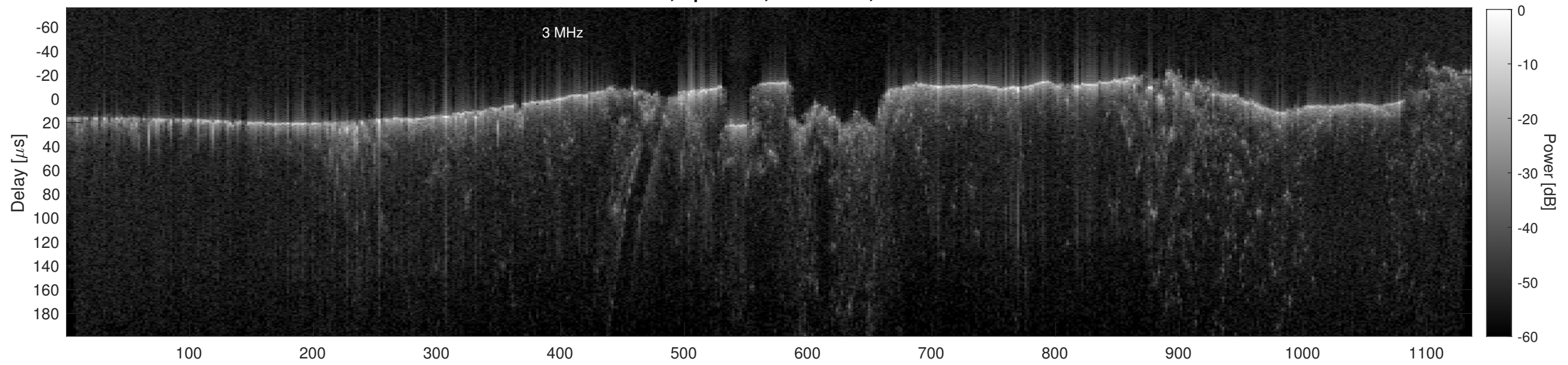
Orbit 19680, Cluttergram
