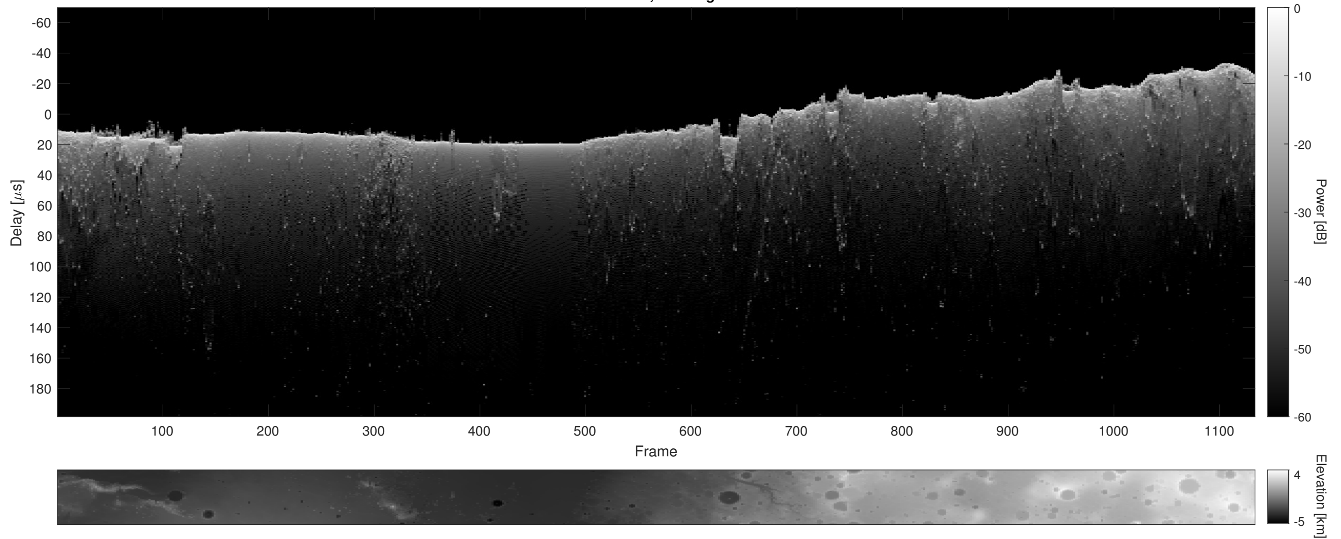
Orbit 19685, Cluttergram
