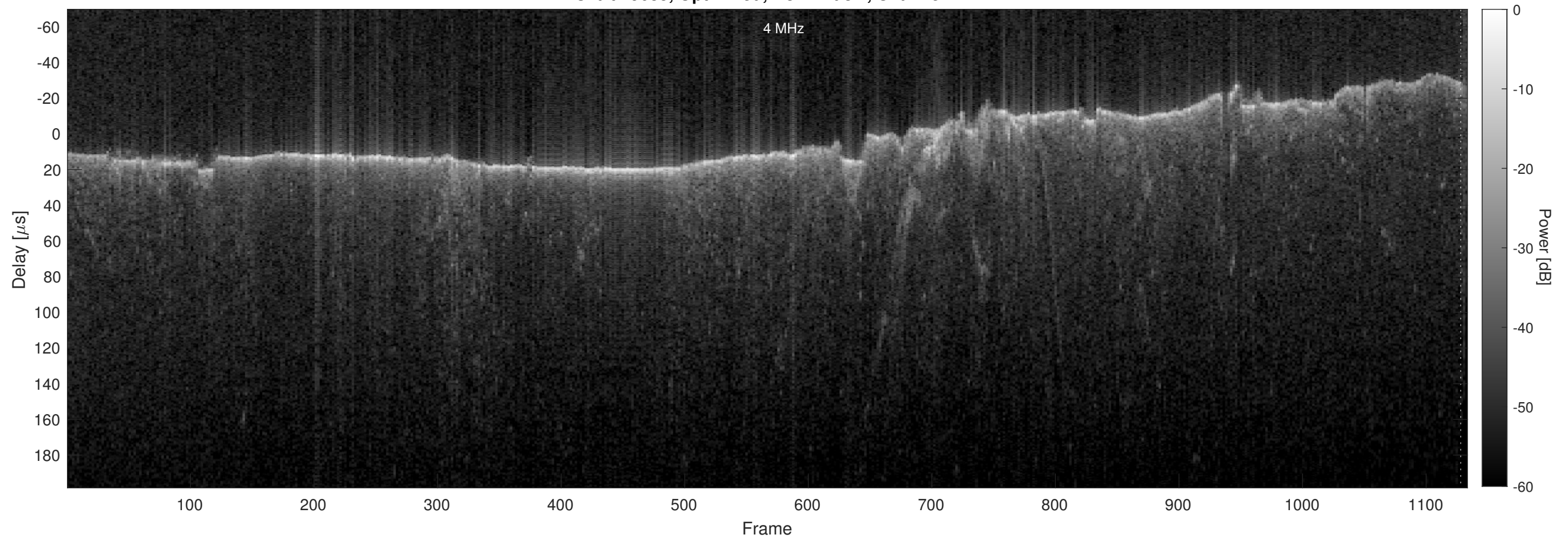
Orbit 19685, Optimized, No Window, Channel 2
