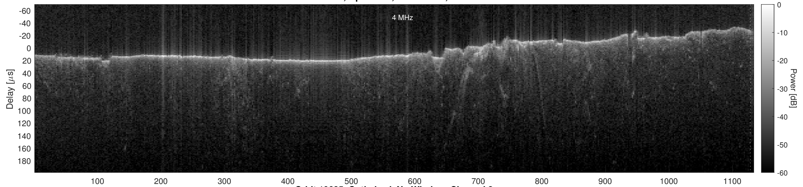
Orbit 19685, Optimized, No Window, Channel 2
