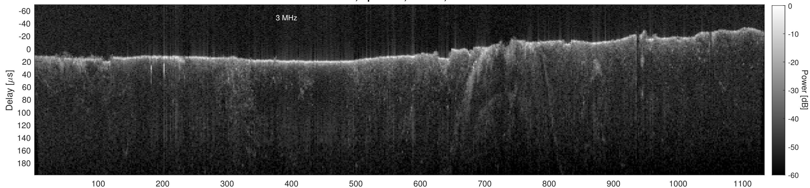
Orbit 19685, Cluttergram
