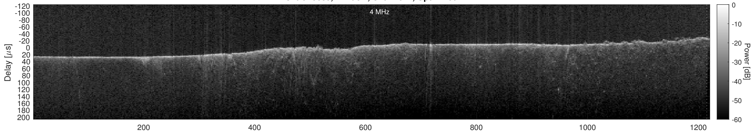
Orbit 19689, Cluttergram
