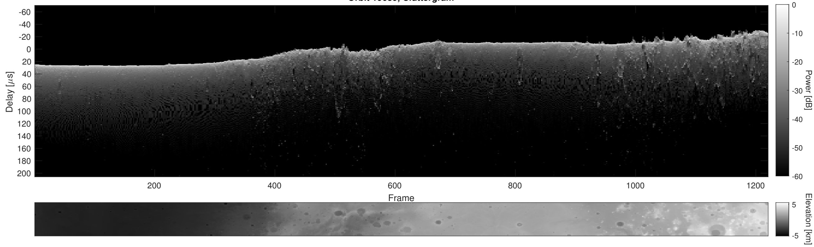
Orbit 19689, Cluttergram
