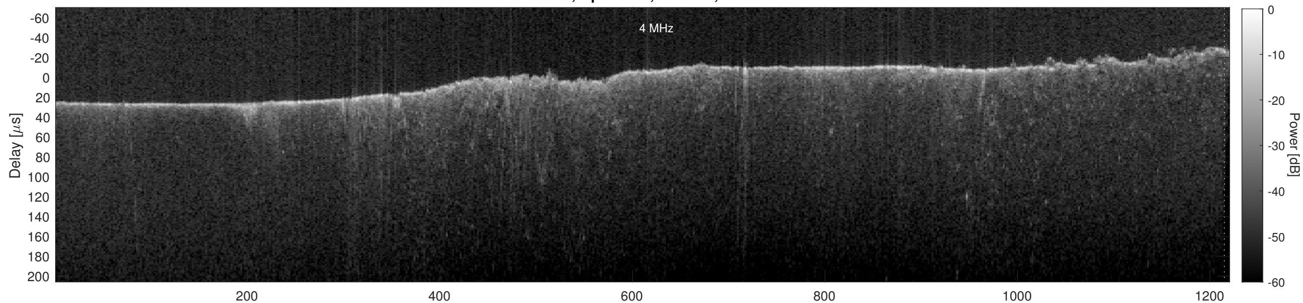
Orbit 19689, Cluttergram
