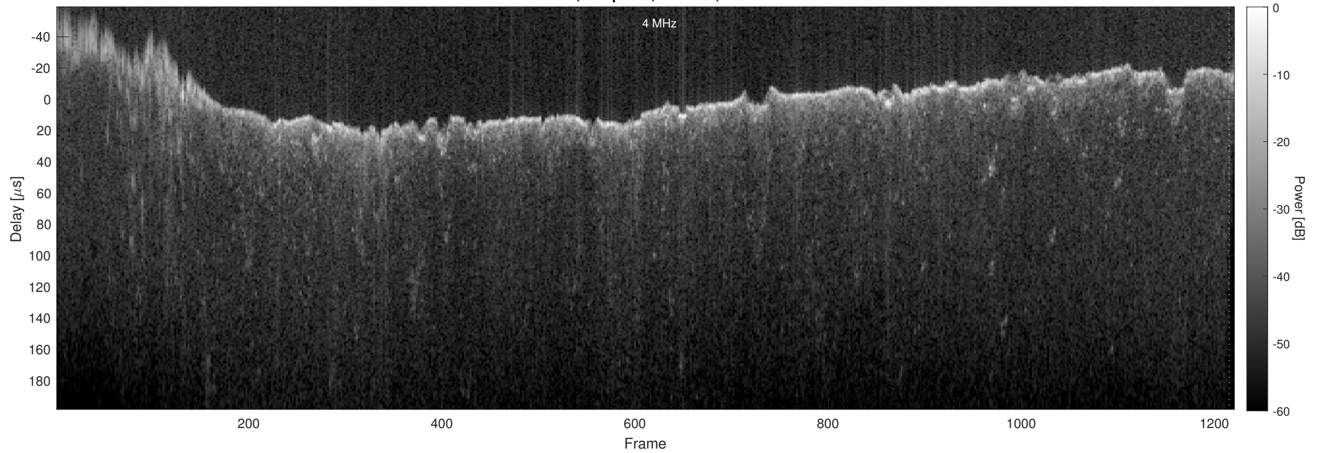
Orbit 19690, Chapman, Window, Channel 2
