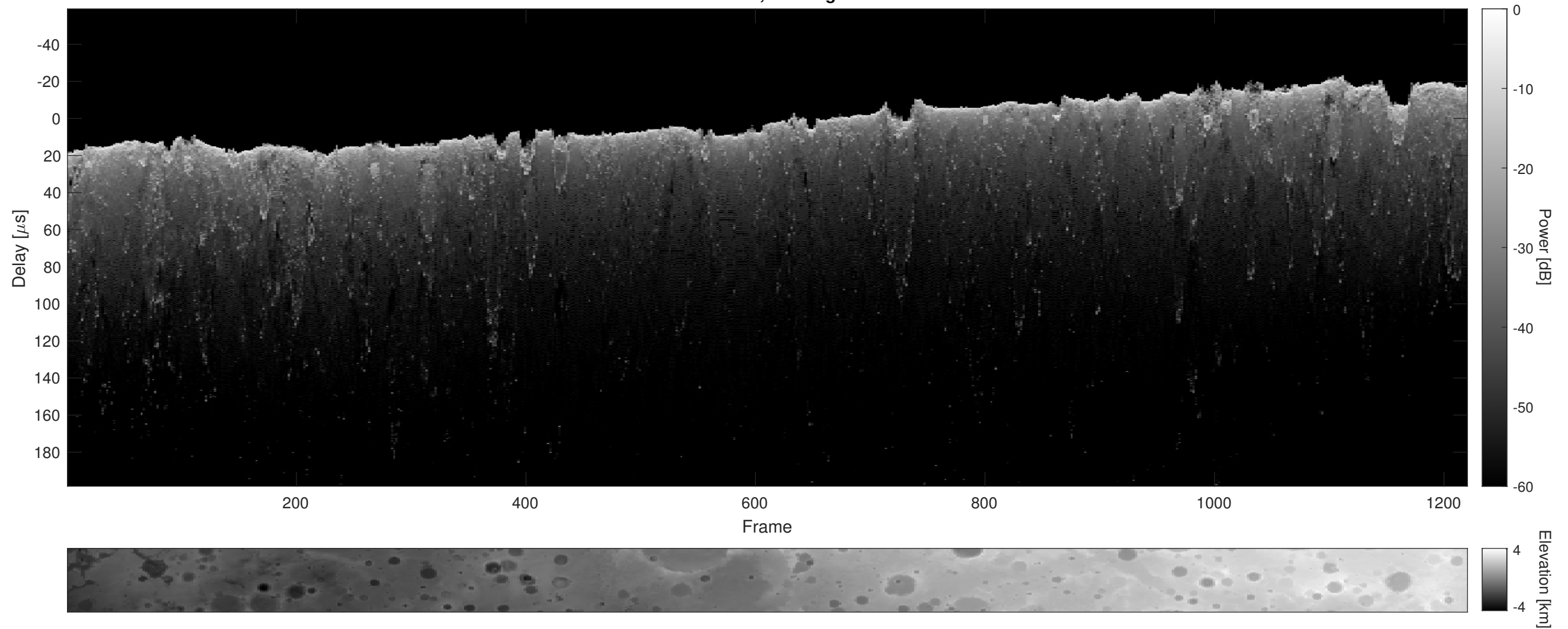
Orbit 19690, Cluttergram
