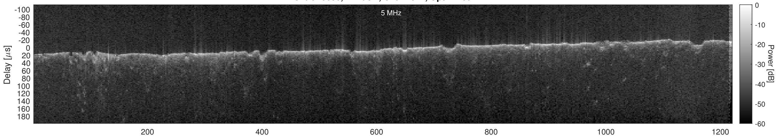
Orbit 19690, Cluttergram
