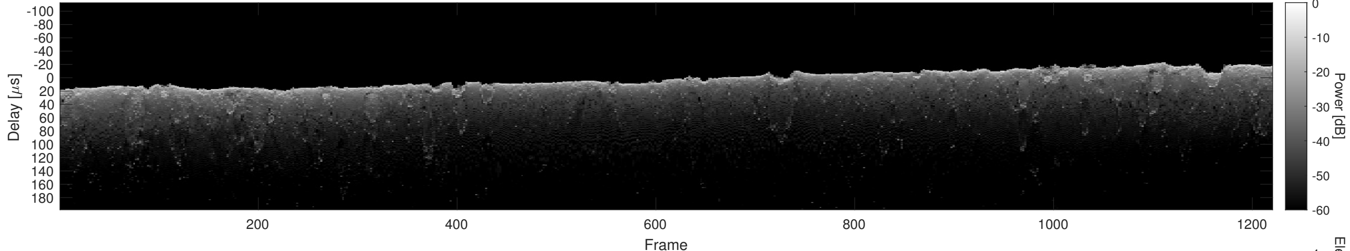
Orbit 19690, Cluttergram
