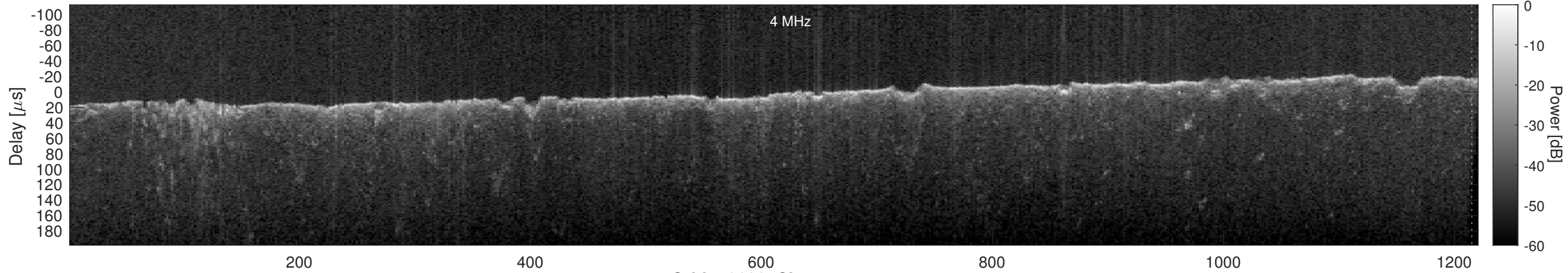
Orbit 19690, Cluttergram
