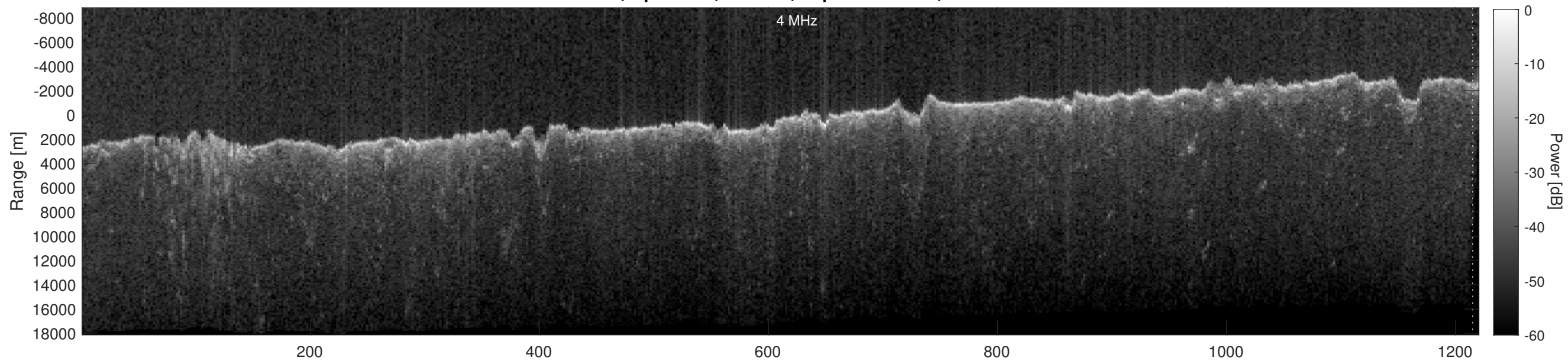
Orbit 19690, Depth-Corrected Cluttergram
