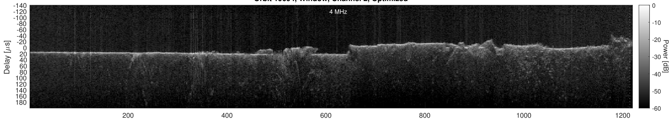
Orbit 19694, Cluttergram
