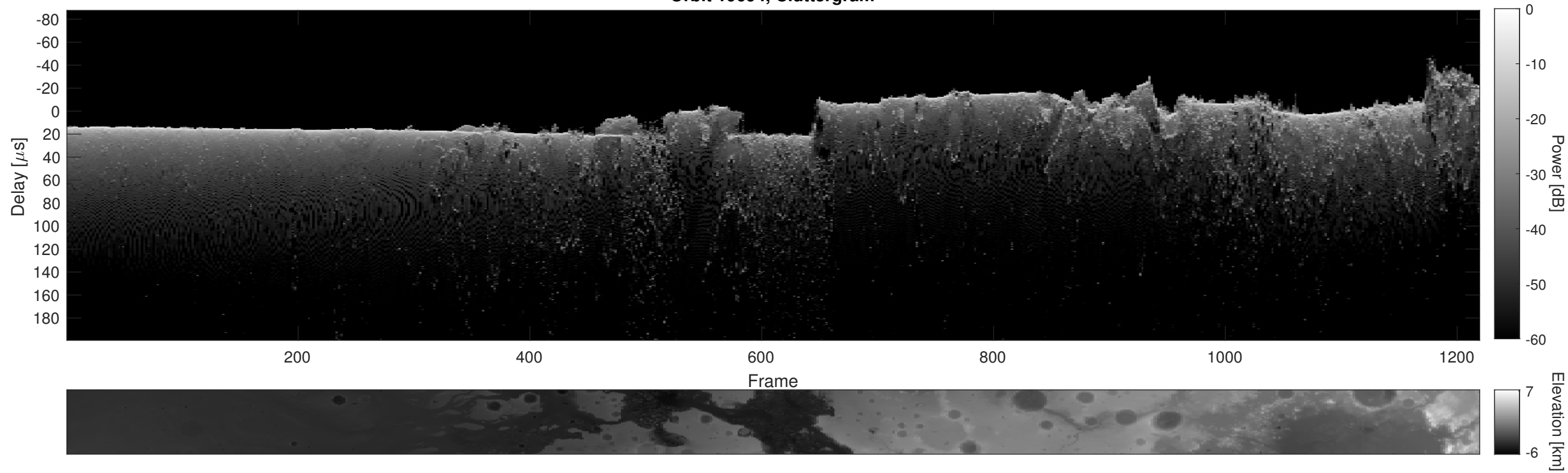
Orbit 19694, Cluttergram
