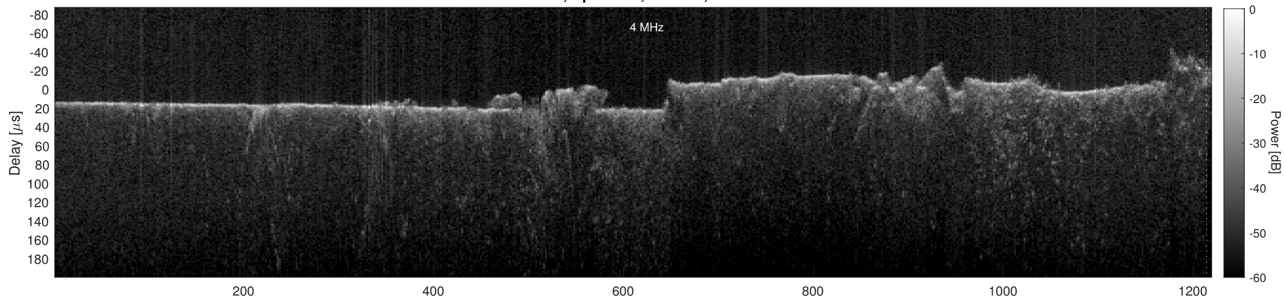
Orbit 19694, Cluttergram
