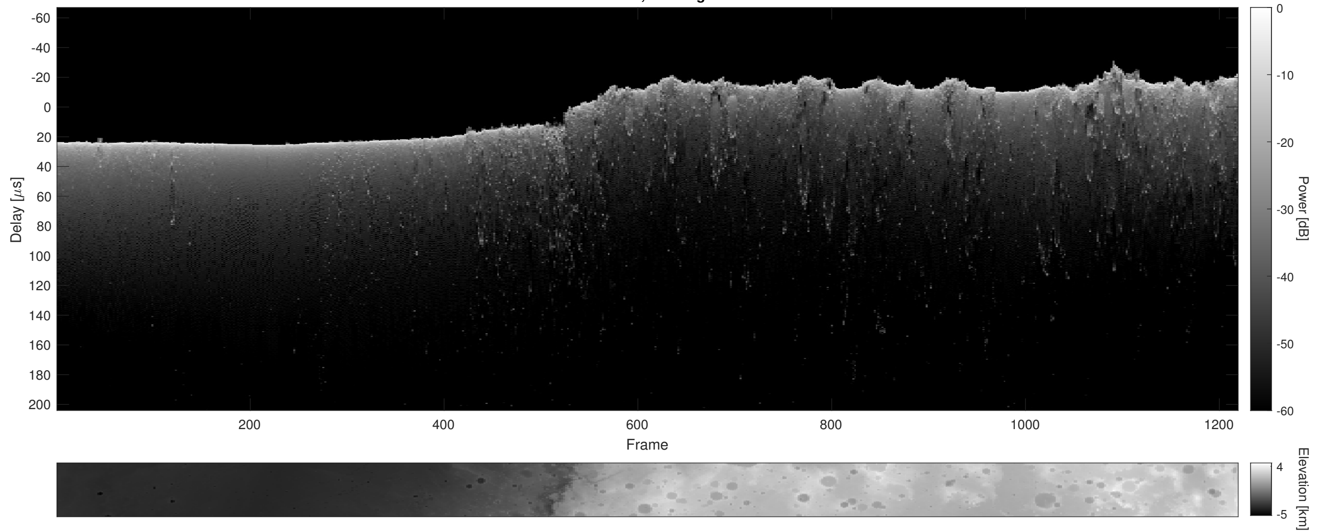
Orbit 19703, Cluttergram
