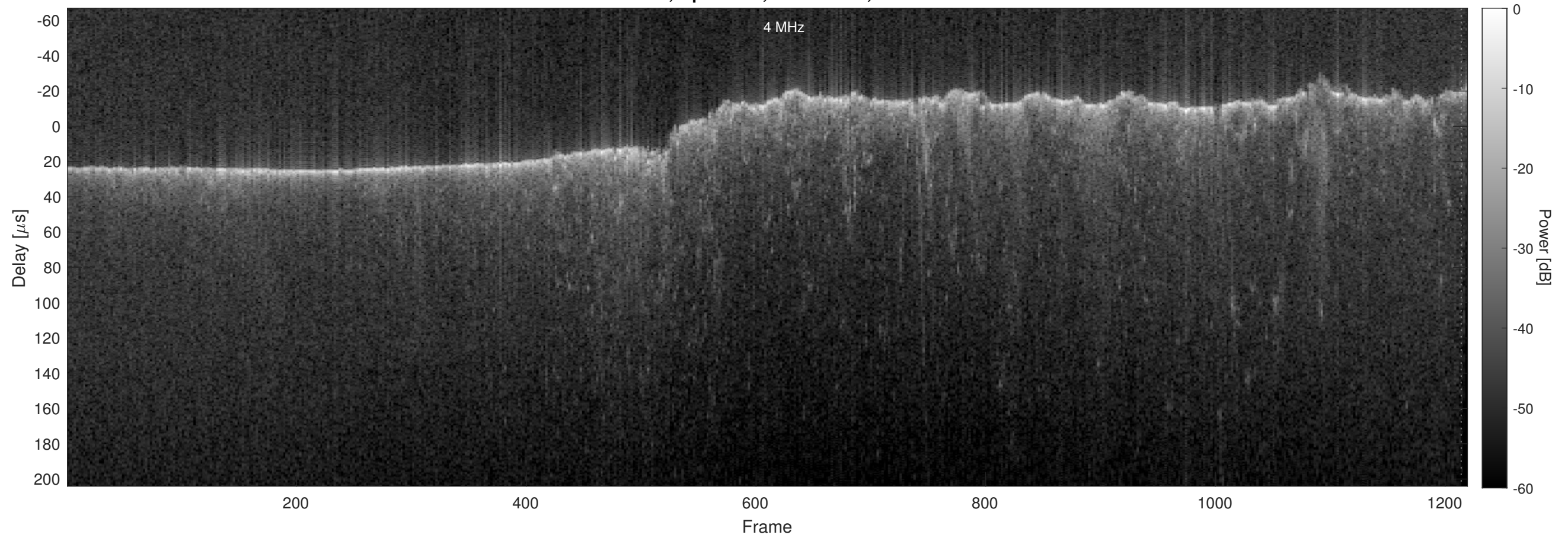
Orbit 19703, Optimized, No Window, Channel 2
