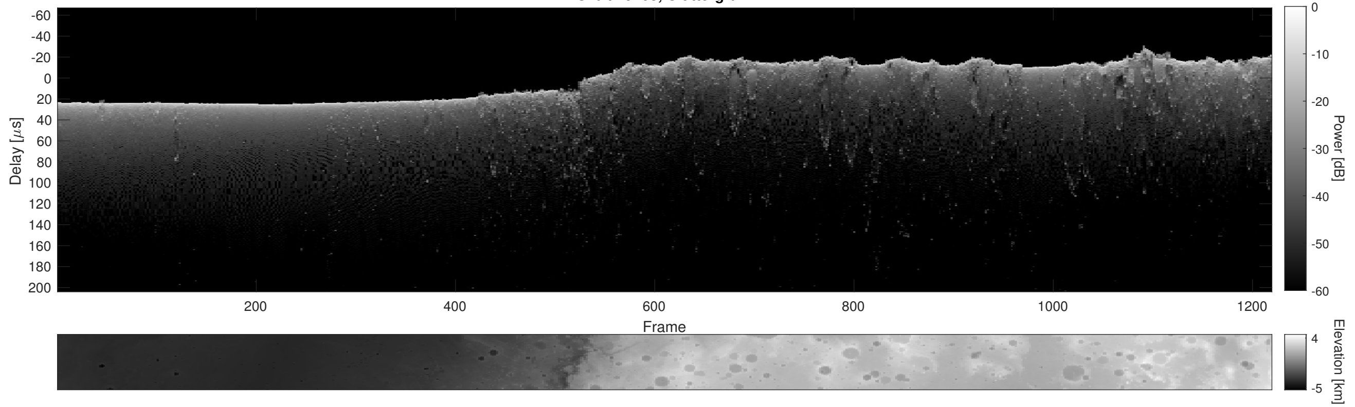
Orbit 19703, Cluttergram
