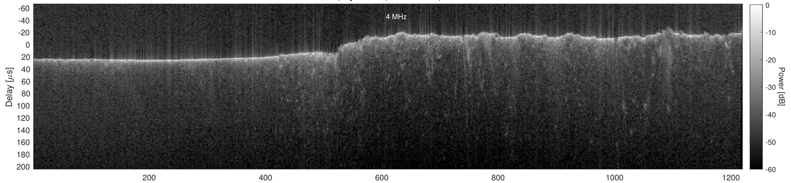
Orbit 19703, Cluttergram
