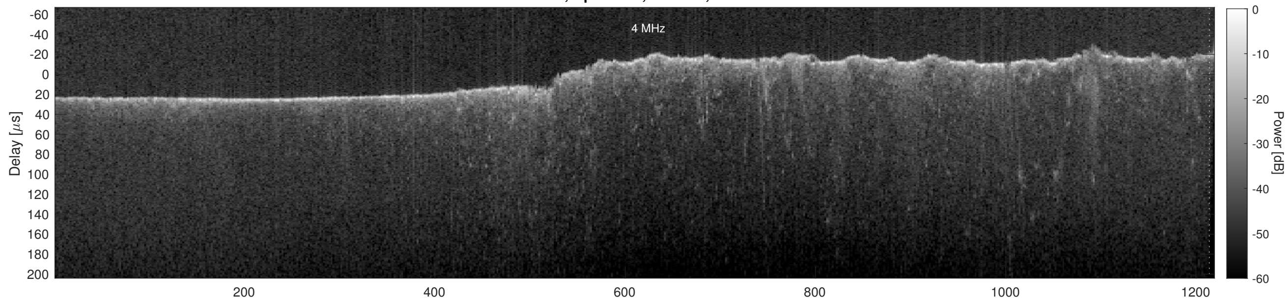
Orbit 19703, Cluttergram
