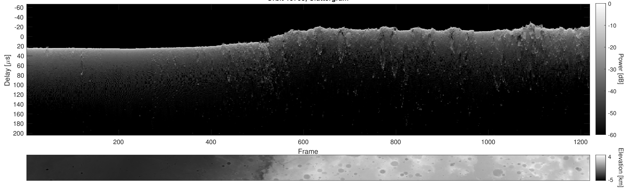
Orbit 19703, Cluttergram
