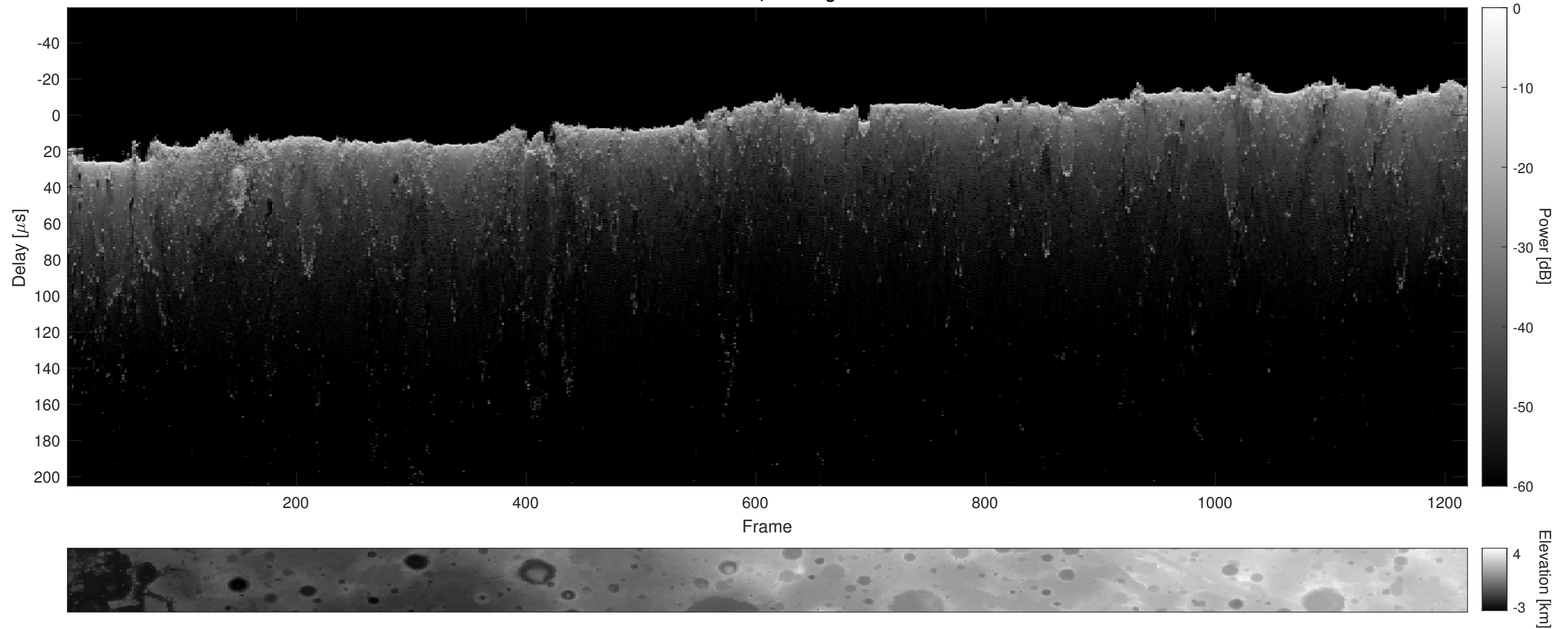
Orbit 19704, Cluttergram
