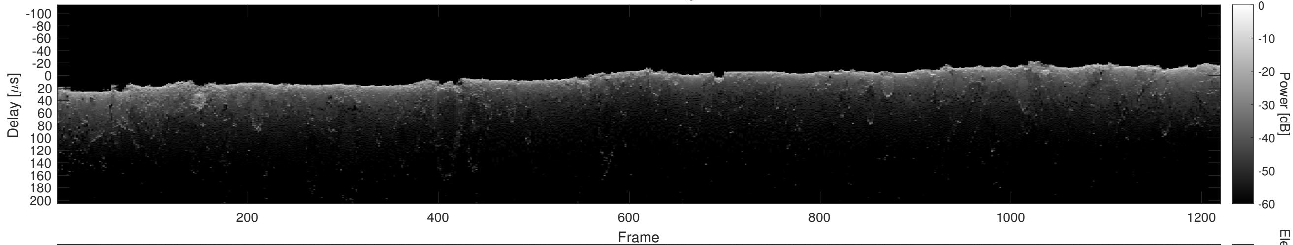
Orbit 19704, Cluttergram
