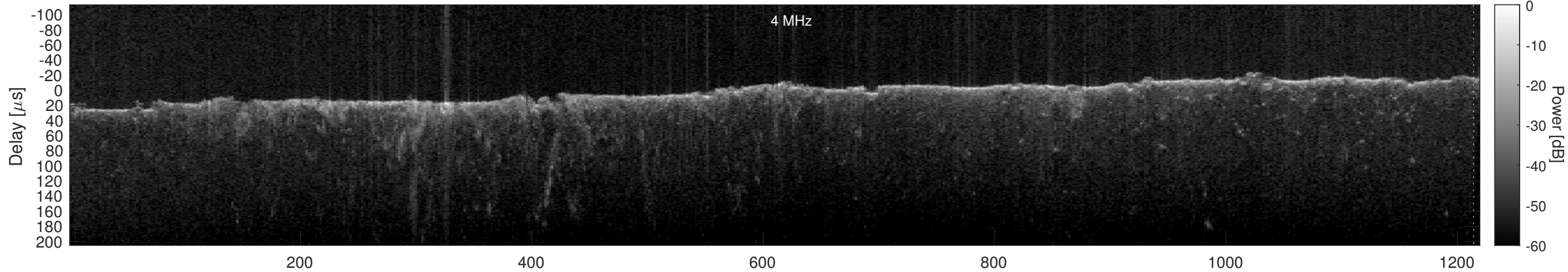
Orbit 19704, Cluttergram
