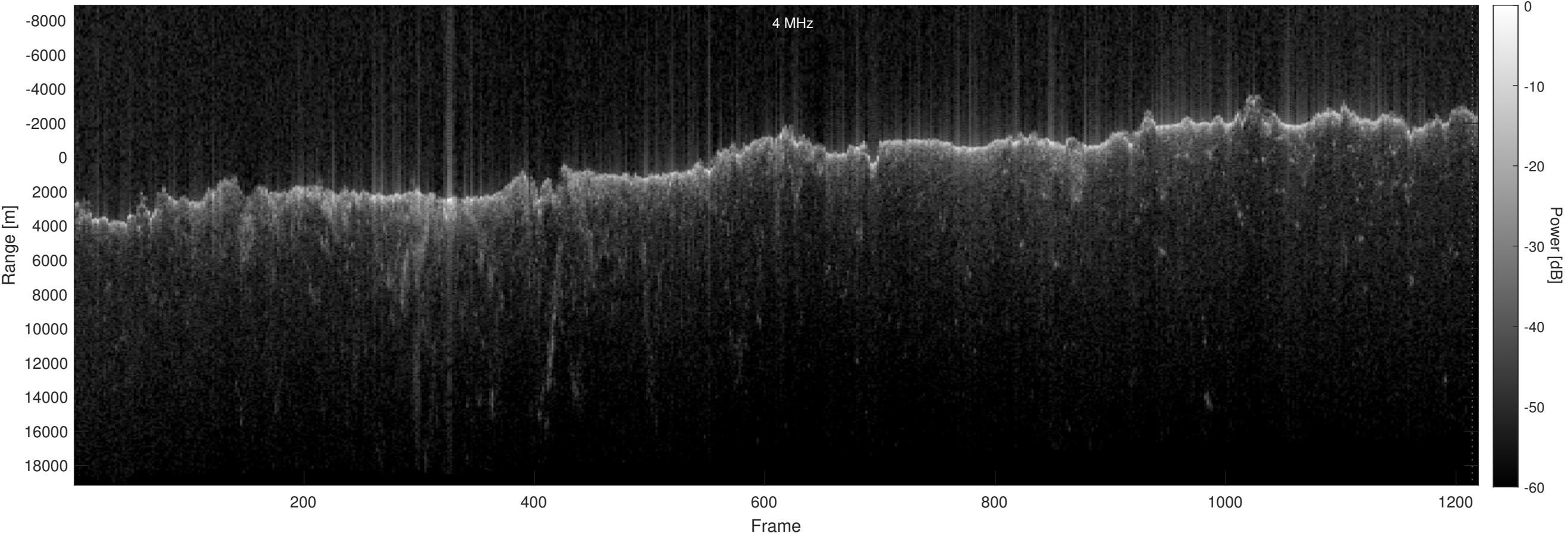
Orbit 19704, Optimized, No Window, Depth-Corrected, Channel 2
