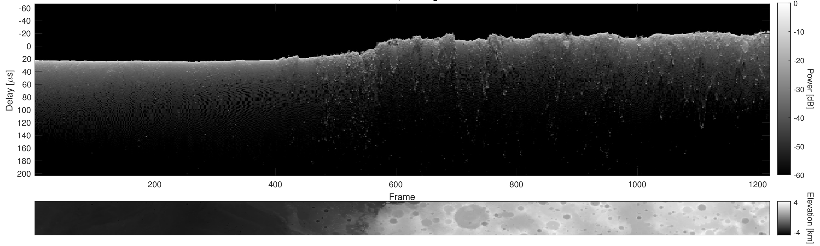
Orbit 19710, Cluttergram
