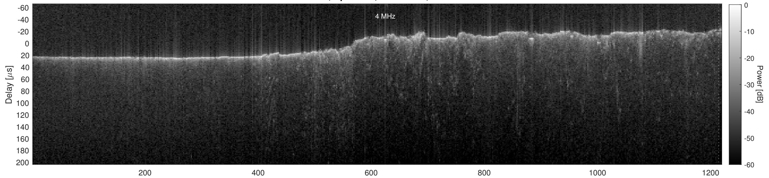
Orbit 19710, Cluttergram
