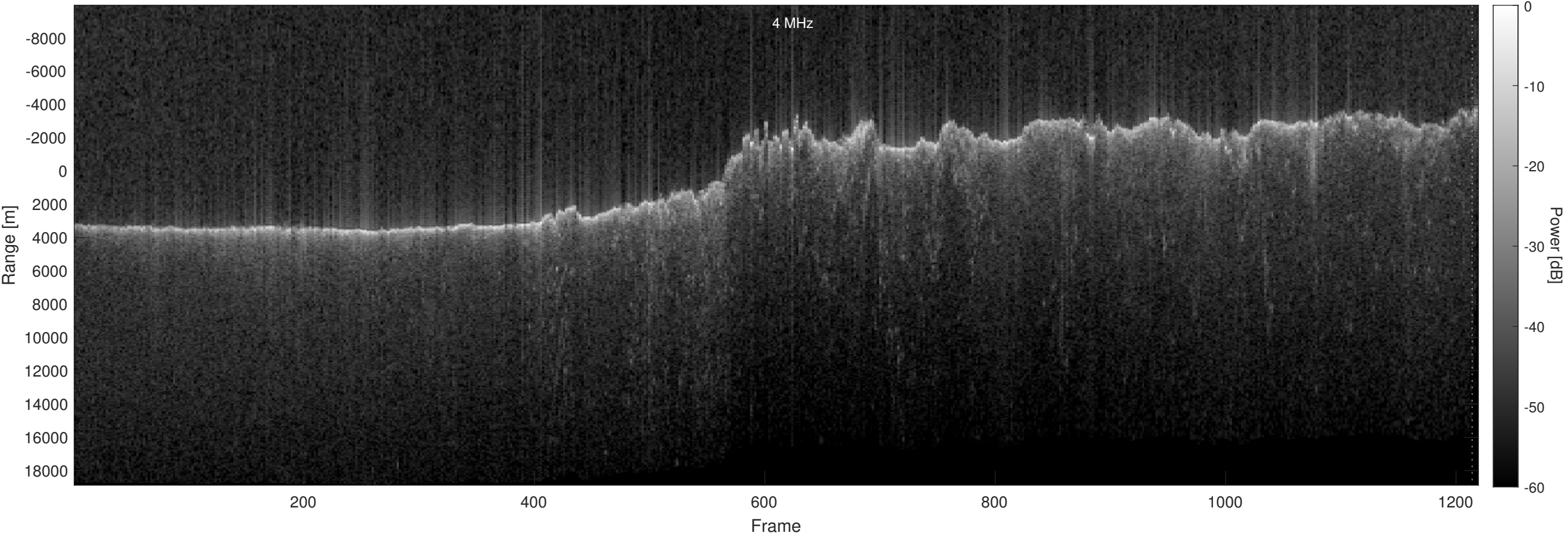
Orbit 19710, Optimized, No Window, Depth-Corrected, Channel 2
