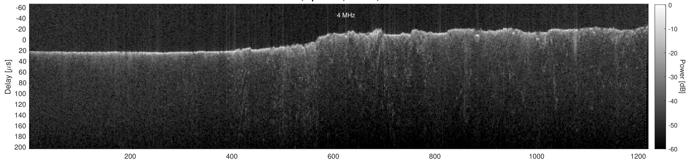
Orbit 19710, Cluttergram
