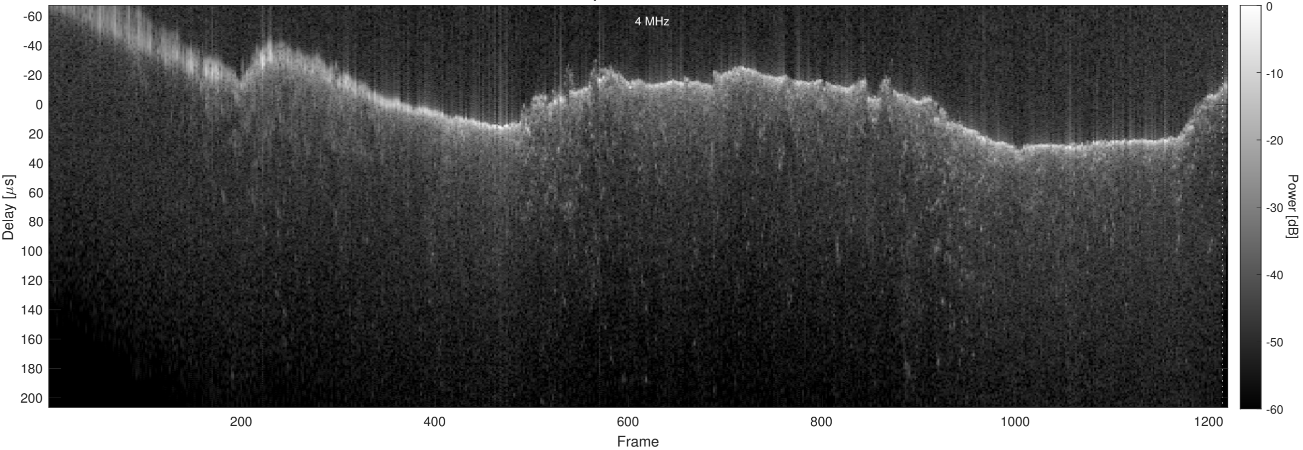
Orbit 19714, Chapman, No Window, Channel 2
