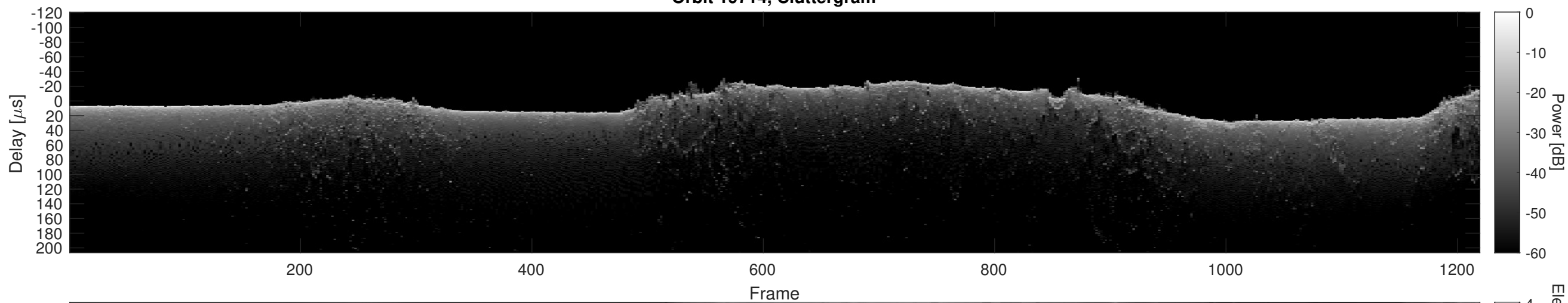
Orbit 19714, Cluttergram
