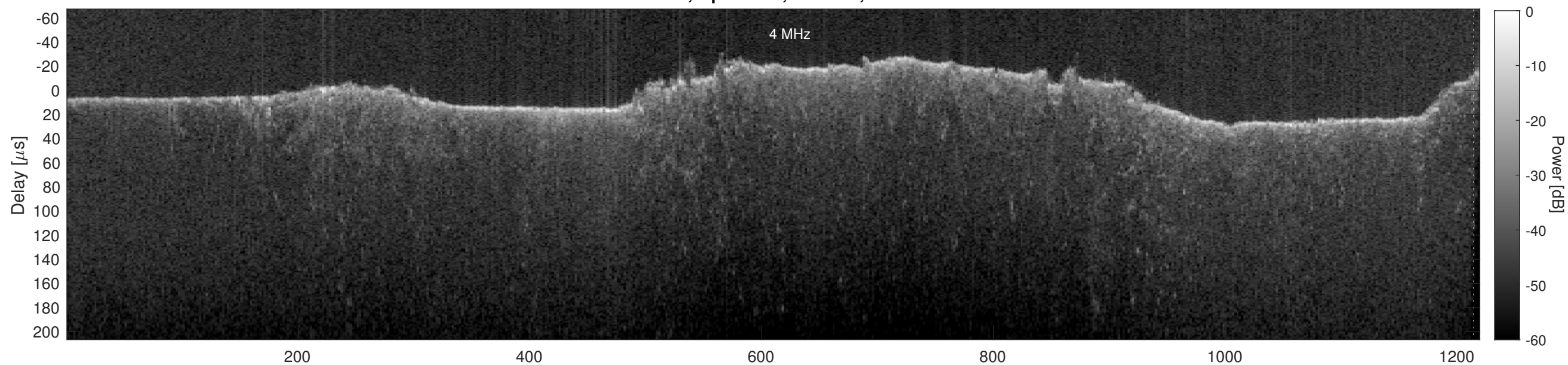
Orbit 19714, Cluttergram
