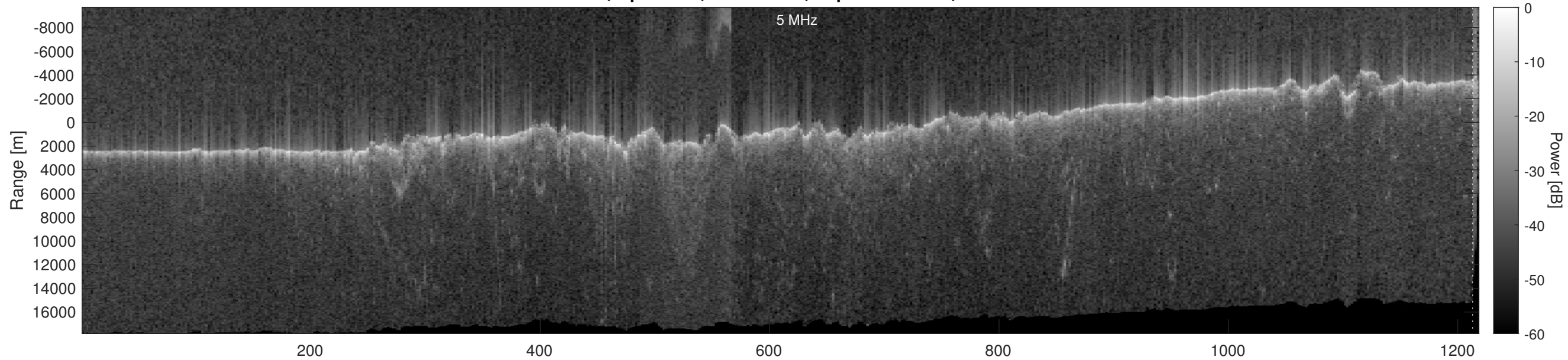
Orbit 19715, Optimized, No Window, Depth-Corrected, Channel 2
