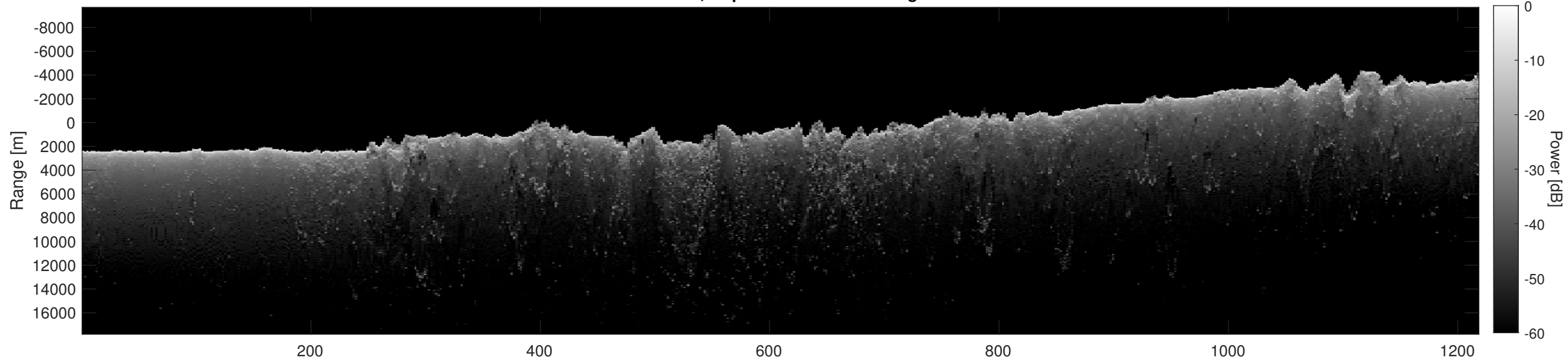
Orbit 19715, Depth-Corrected Cluttergram
