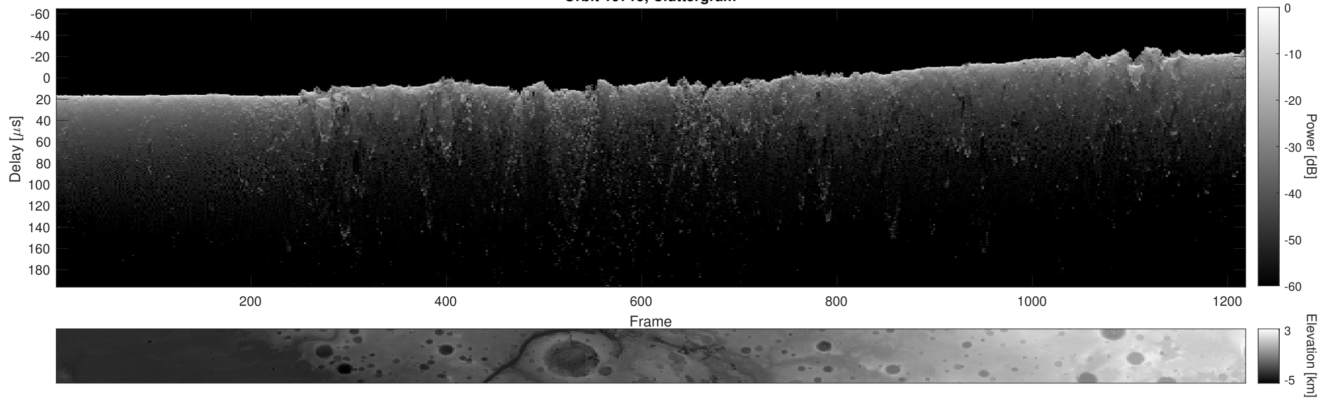
Orbit 19715, Cluttergram
