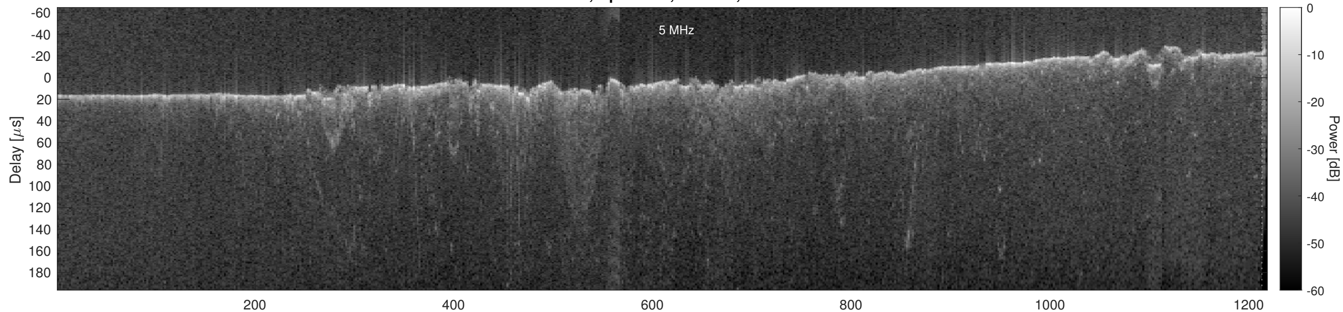
Orbit 19715, Optimized, Window, Channel 2
