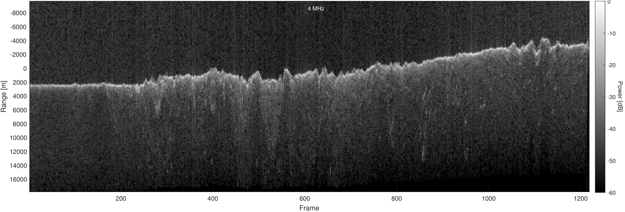
Orbit 19715, Optimized, Window, Depth-Corrected, Channel 2
