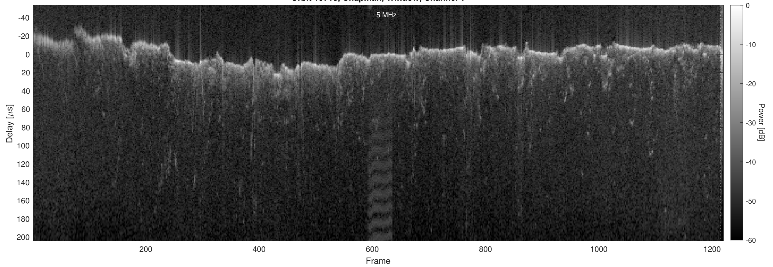
Orbit 19718, Chapman, Window, Channel 2
