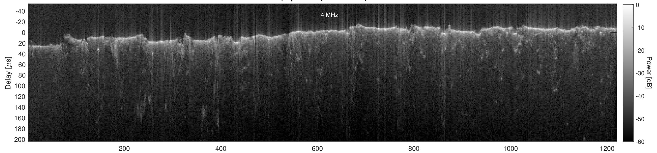
Orbit 19718, Cluttergram
