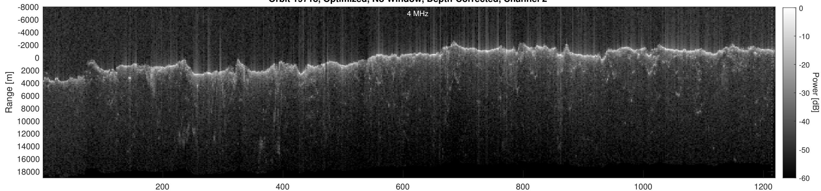
Orbit 19718, Depth-Corrected Cluttergram
