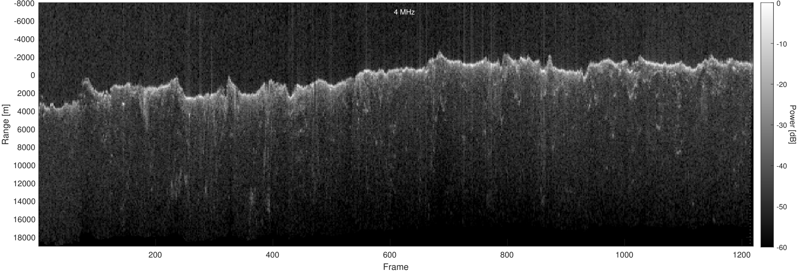
Orbit 19718, Optimized, Window, Depth-Corrected, Channel 2
