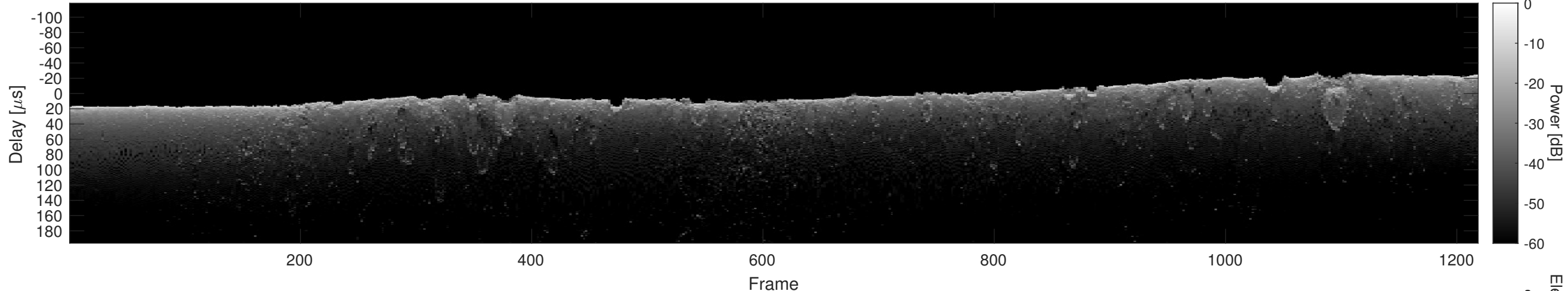
Orbit 19722, Cluttergram
