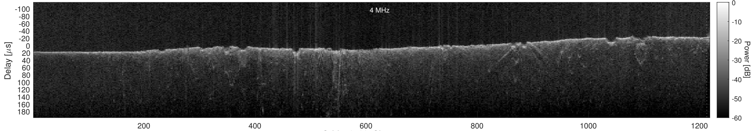
Orbit 19722, Cluttergram
