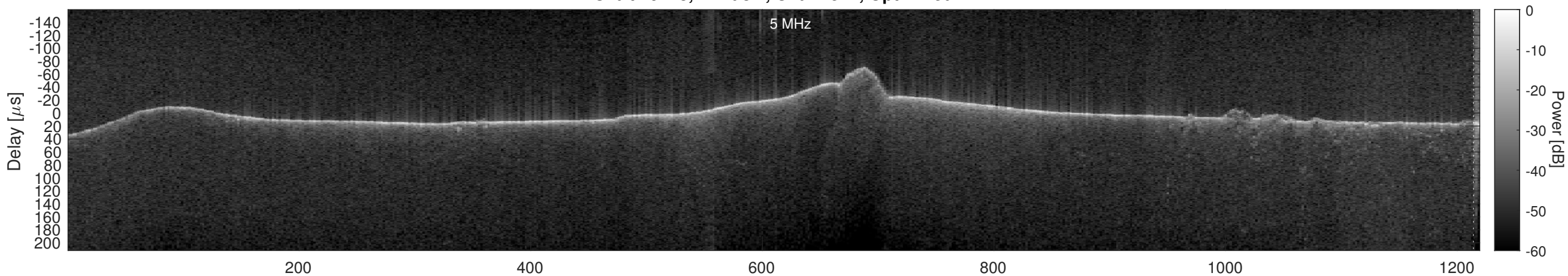
Orbit 19723, Cluttergram
